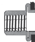
3. BLIND NUT INSTALLED WITH STANDARD HEAD CONFIGURATION.
