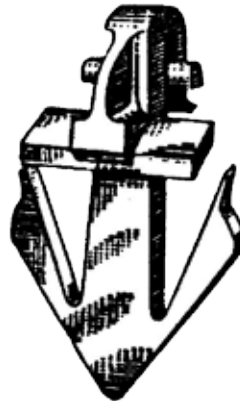
445685 20632190 Garnish Mldg. Clip Rear, Upper & Side GM Box Qty. 10
